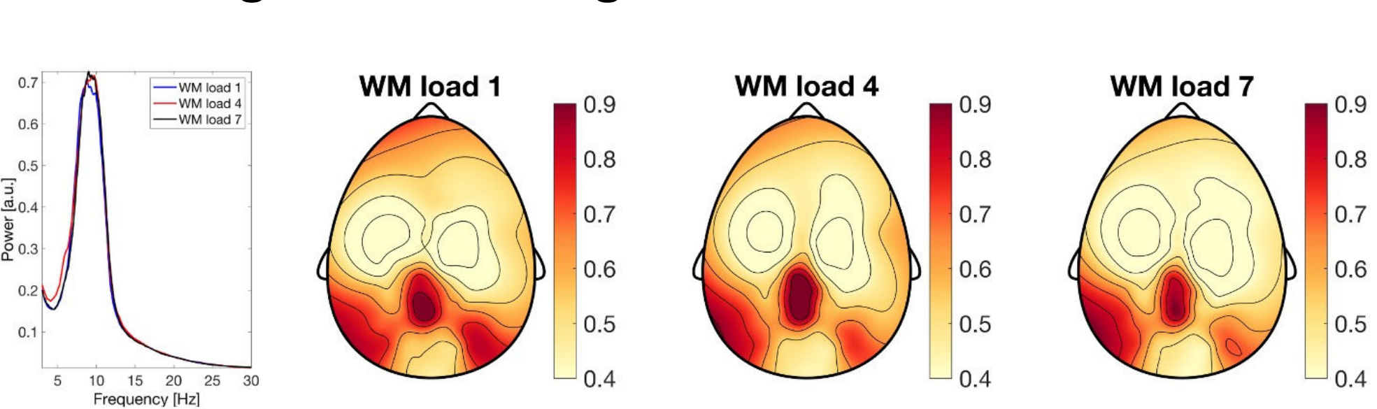
Fig. 5: Grand average occipital power spectra and topographical alpha power distribution across WM load condition 1, 4 and 7.
